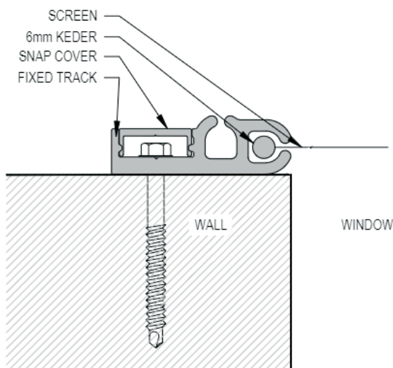
1 SECTION - FACE MOUNT SCALE: 12" = 1'-0"
