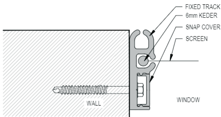
2 SECTION - INSIDE MOUNT SCALE: 12" = 1'-0"
